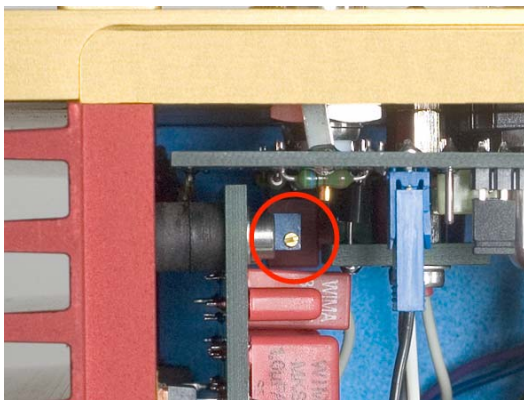
Fig.9 – DC Offset Trimmer
