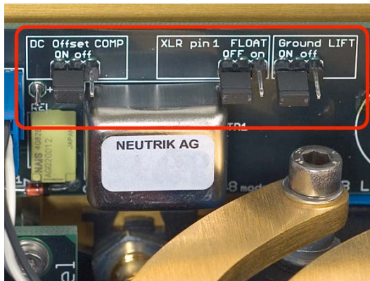
Fig.3 – Jumpers
