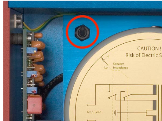
Fig.2 – Speaker's impedance switch
